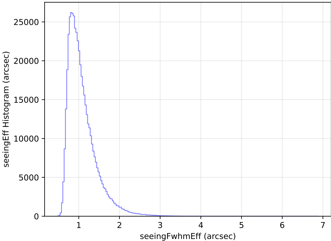
mw_roll_bulge_v3.3_10yrs All sky i band: seeingEff Histogram
