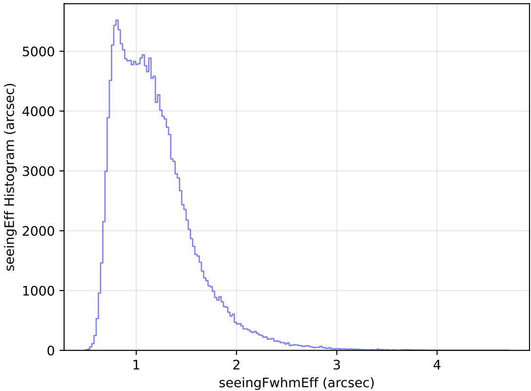
mw_roll_bulge_v3.3_10yrs All sky g band: seeingEff Histogram
