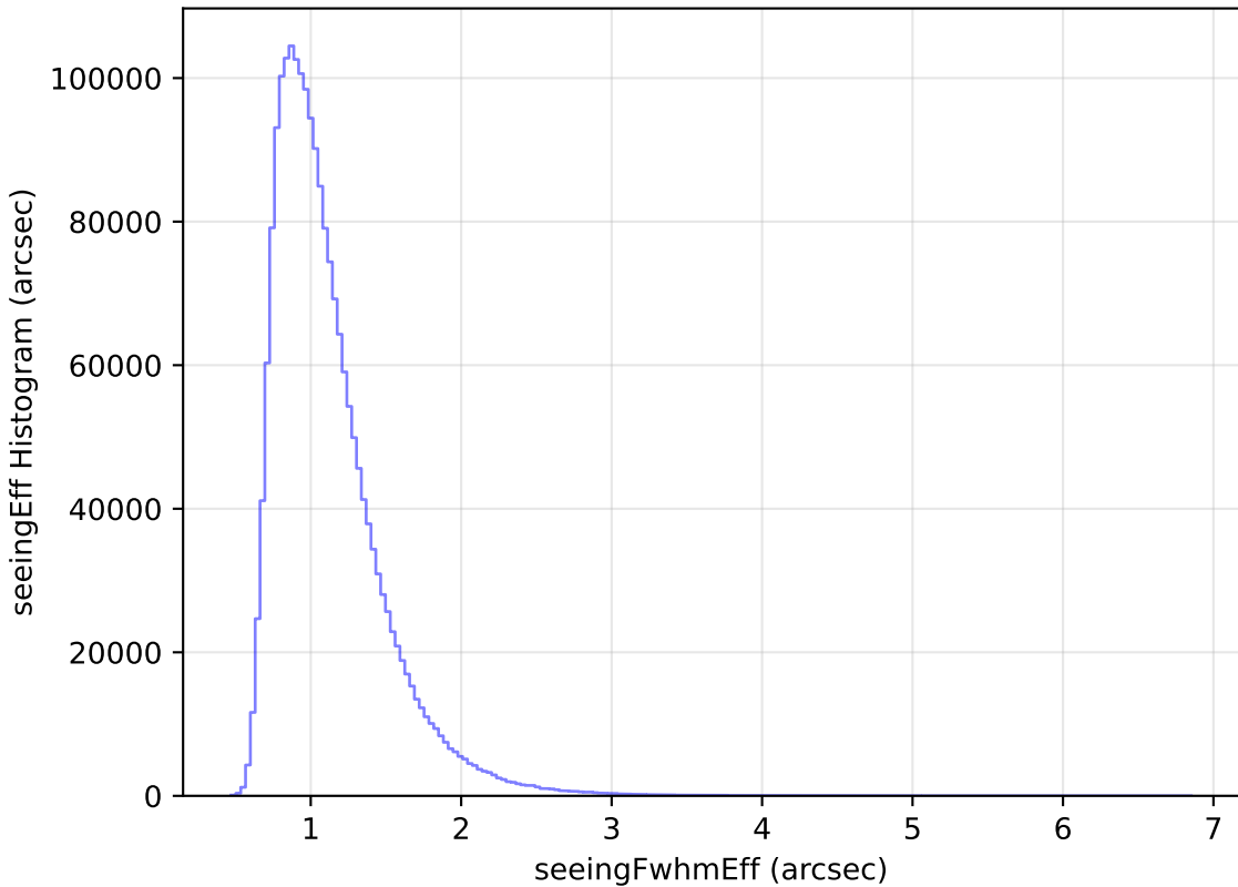
mw_roll_bulge_v3.3_10yrs All sky all bands: seeingEff Histogram
