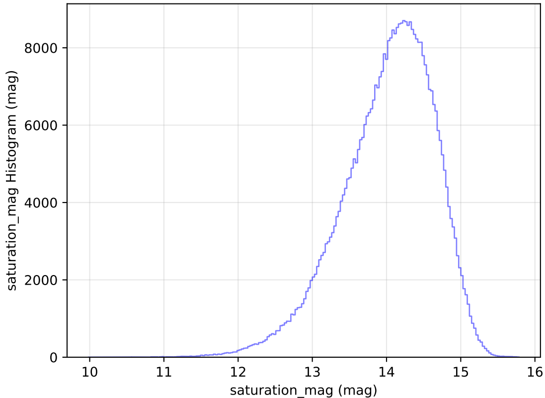
mw_roll_bulge_v3.3_10yrs WFD z band: saturation_mag Histogram
