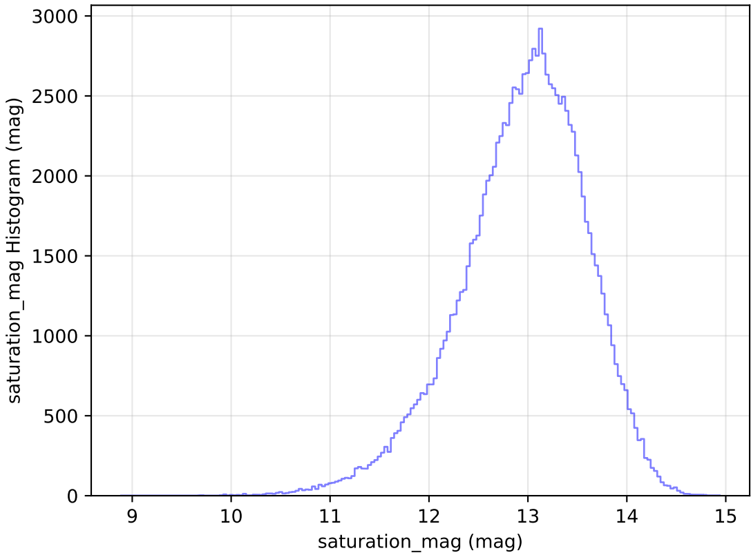
mw_roll_bulge_v3.3_10yrs WFD u band: saturation_mag Histogram
