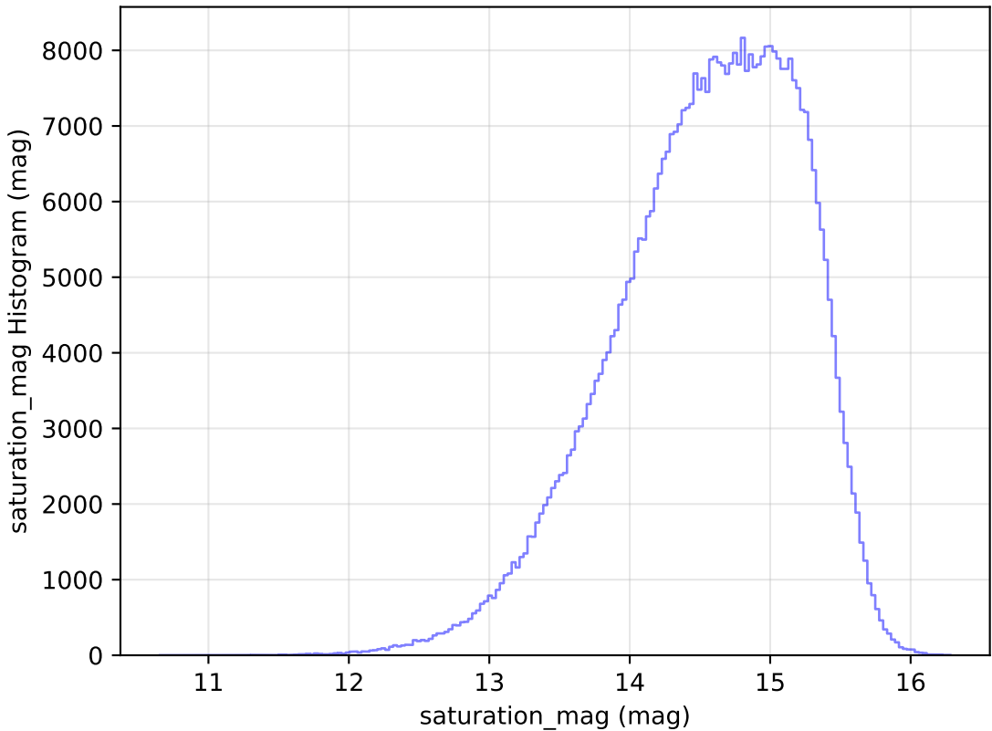
mw_roll_bulge_v3.3_10yrs WFD r band: saturation_mag Histogram
