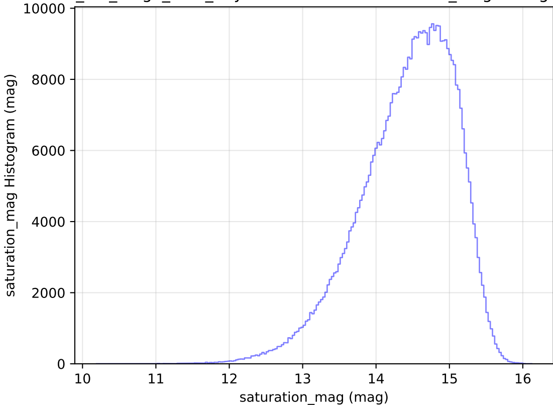
mw_roll_bulge_v3.3_10yrs WFD i band: saturation_mag Histogram
