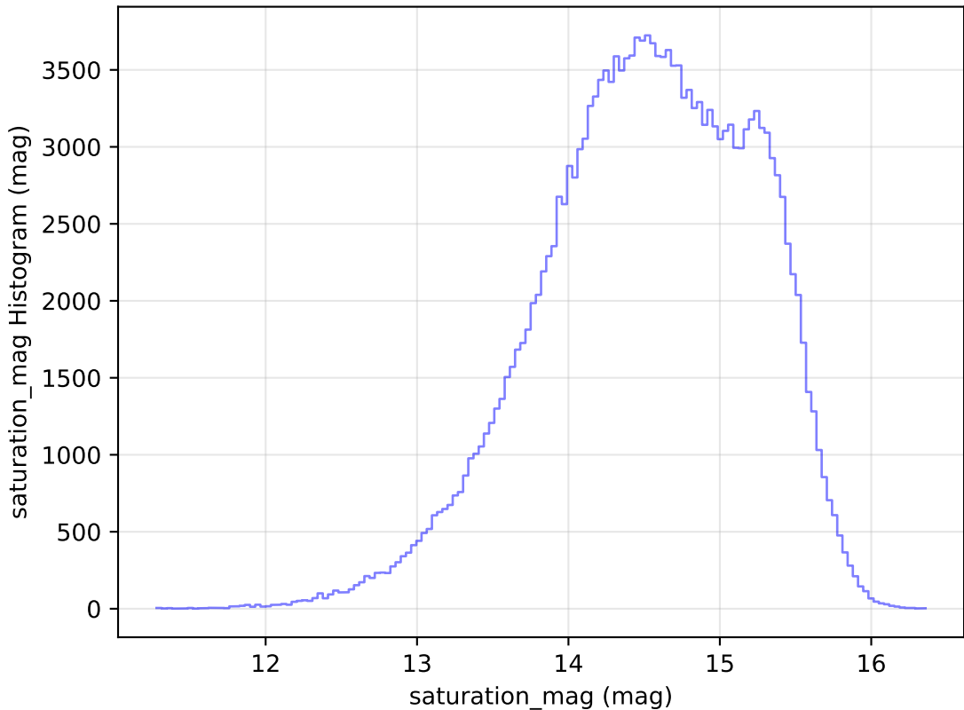
mw_roll_bulge_v3.3_10yrs WFD g band: saturation_mag Histogram
