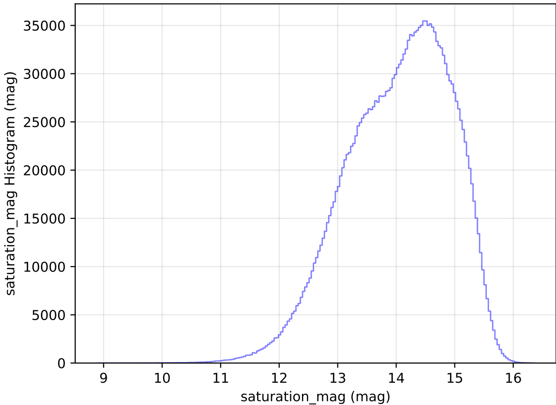
mw_roll_bulge_v3.3_10yrs WFD all bands: saturation_mag Histogram
