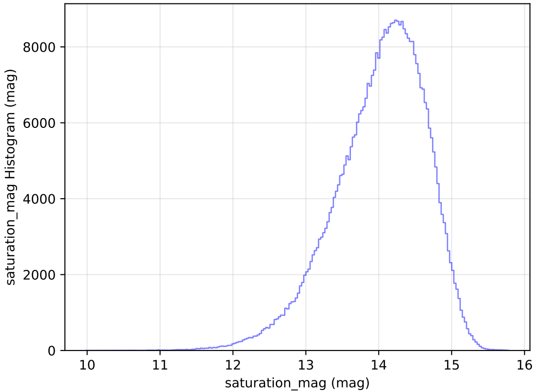
mw_roll_bulge_v3.3_10yrs All sky z band: saturation_mag Histogram
