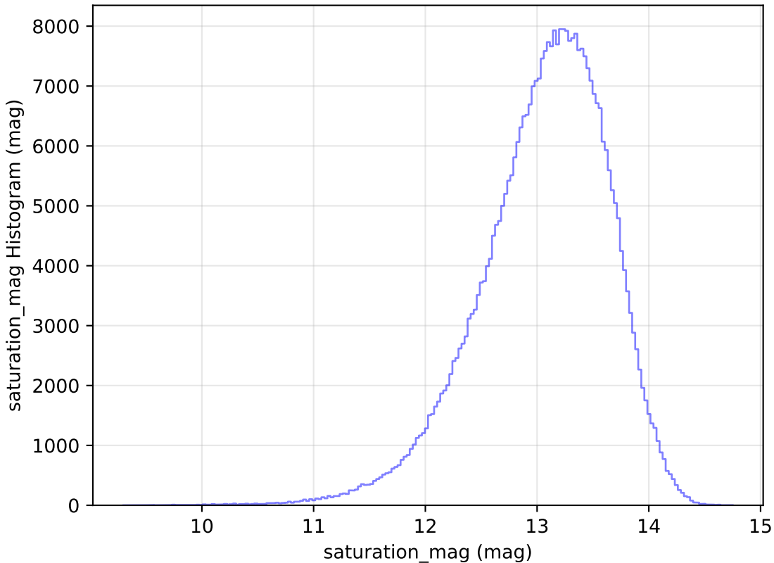
mw_roll_bulge_v3.3_10yrs All sky y band: saturation_mag Histogram
