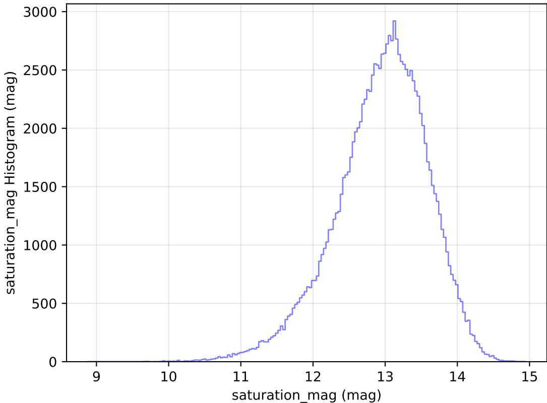
mw_roll_bulge_v3.3_10yrs All sky u band: saturation_mag Histogram
