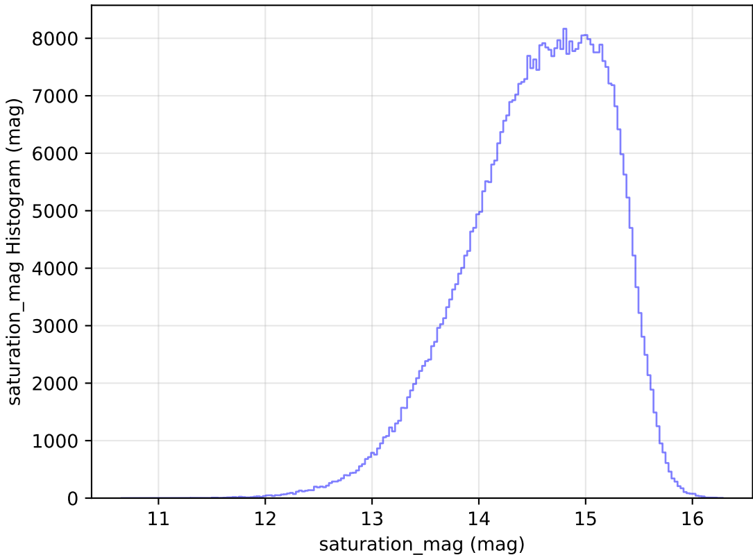
mw_roll_bulge_v3.3_10yrs All sky r band: saturation_mag Histogram
