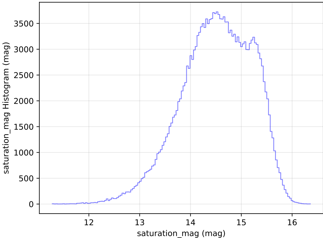
mw_roll_bulge_v3.3_10yrs All sky g band: saturation_mag Histogram
