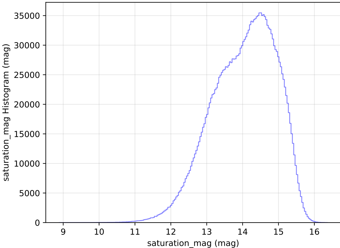
mw_roll_bulge_v3.3_10yrs All sky all bands: saturation_mag Histogram
