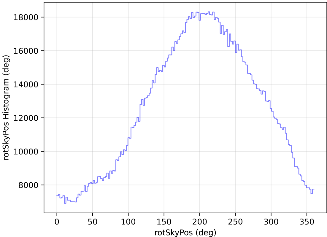
mw_roll_bulge_v3.3_10yrs WFD all bands: rotSkyPos Histogram
