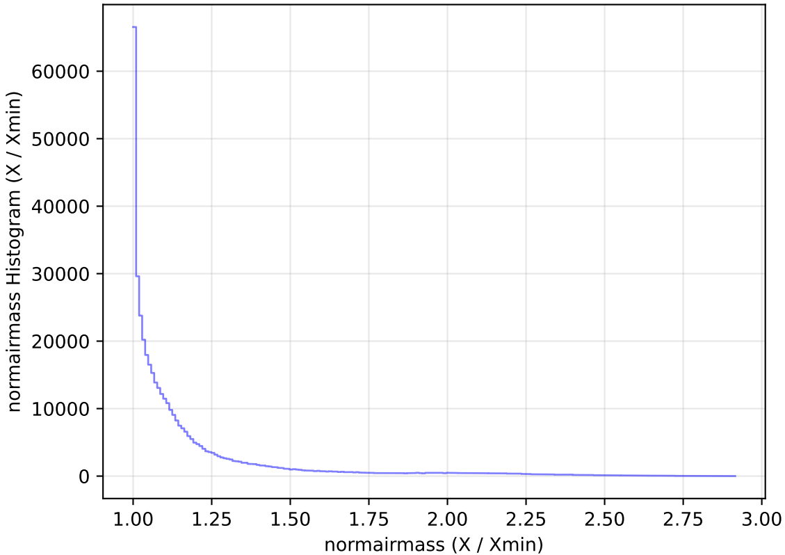
mw_roll_bulge_v3.3_10yrs WFD z band: normairmass Histogram
