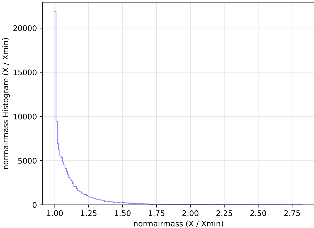
mw_roll_bulge_v3.3_10yrs WFD u band: normairmass Histogram
