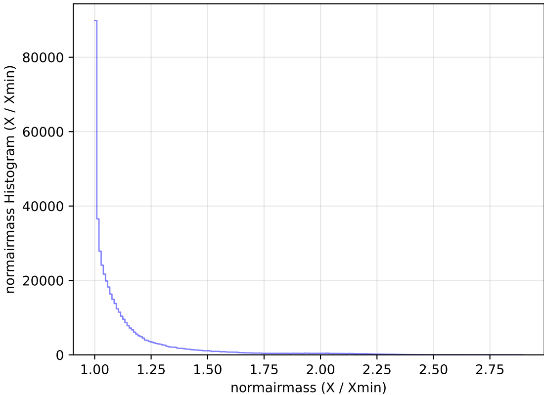
mw_roll_bulge_v3.3_10yrs WFD r band: normairmass Histogram
