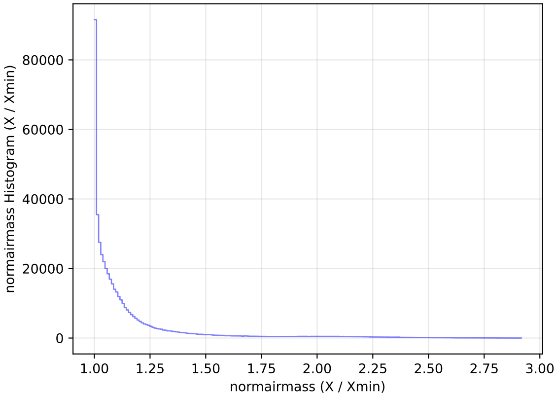
mw_roll_bulge_v3.3_10yrs WFD i band: normairmass Histogram
