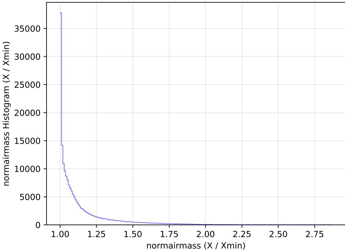
mw_roll_bulge_v3.3_10yrs WFD g band: normairmass Histogram
