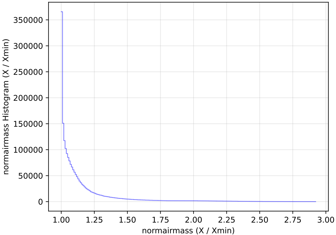
mw_roll_bulge_v3.3_10yrs WFD all bands: normairmass Histogram
