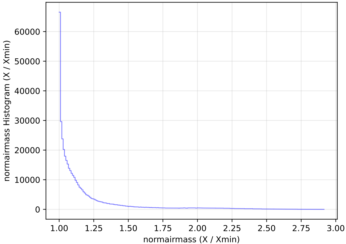
mw_roll_bulge_v3.3_10yrs All sky z band: normairmass Histogram
