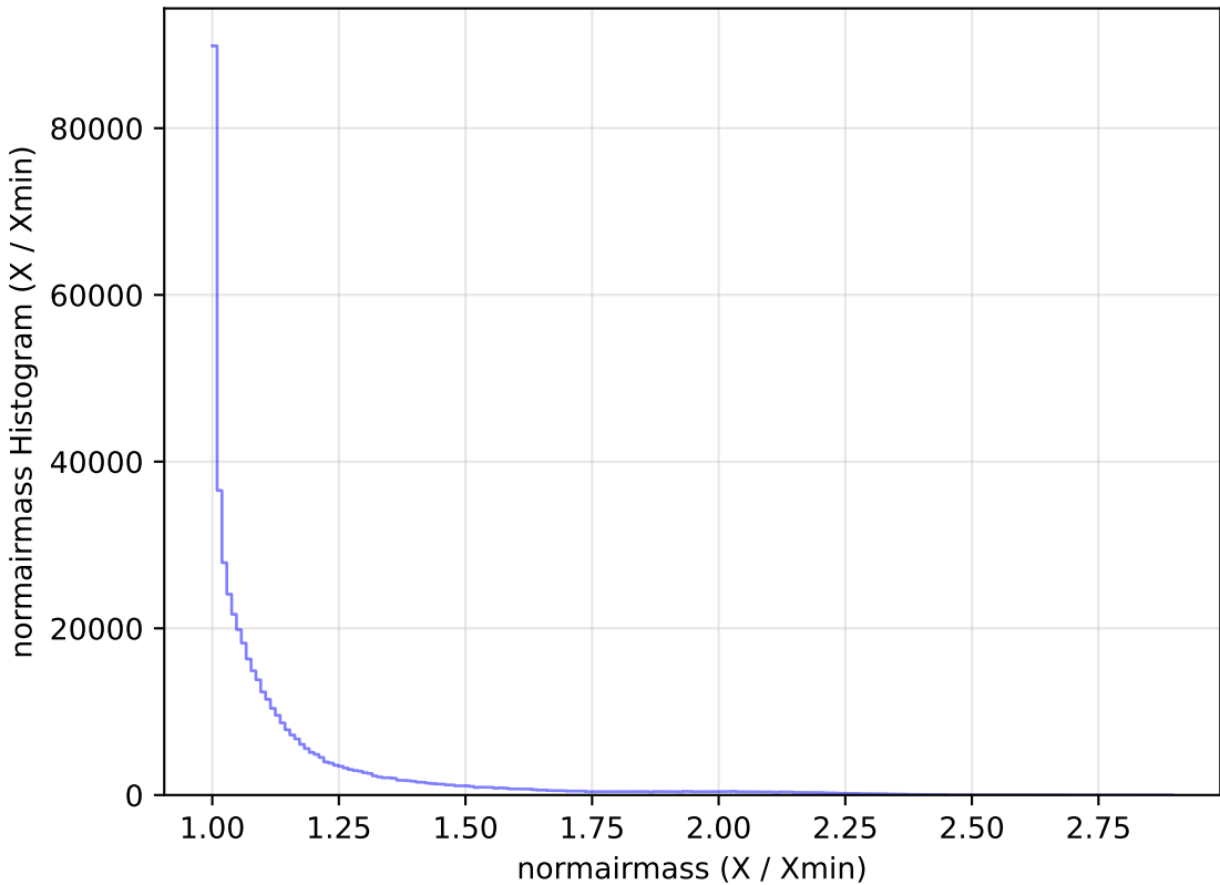
mw_roll_bulge_v3.3_10yrs All sky r band: normairmass Histogram
