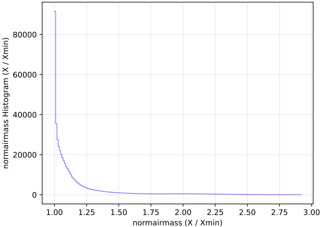
mw_roll_bulge_v3.3_10yrs All sky i band: normairmass Histogram
