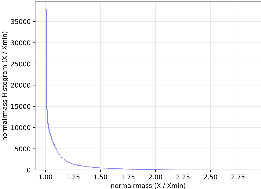
mw_roll_bulge_v3.3_10yrs All sky g band: normairmass Histogram
