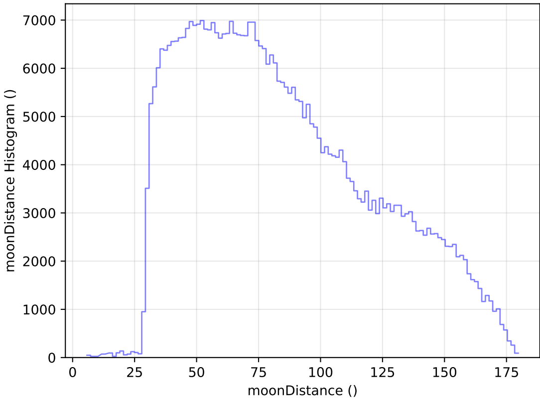
mw_roll_bulge_v3.3_10yrs WFD z band: moonDistance Histogram
