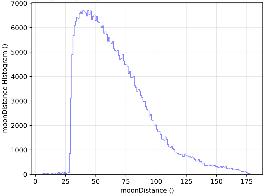
mw_roll_bulge_v3.3_10yrs WFD y band: moonDistance Histogram
