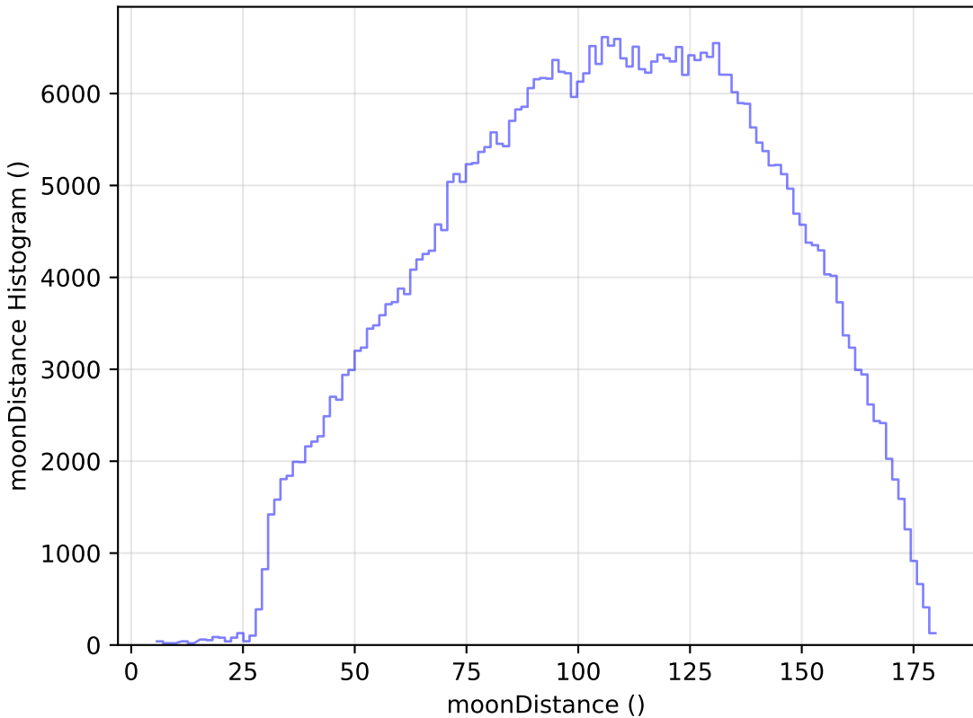
mw_roll_bulge_v3.3_10yrs WFD r band: moonDistance Histogram
