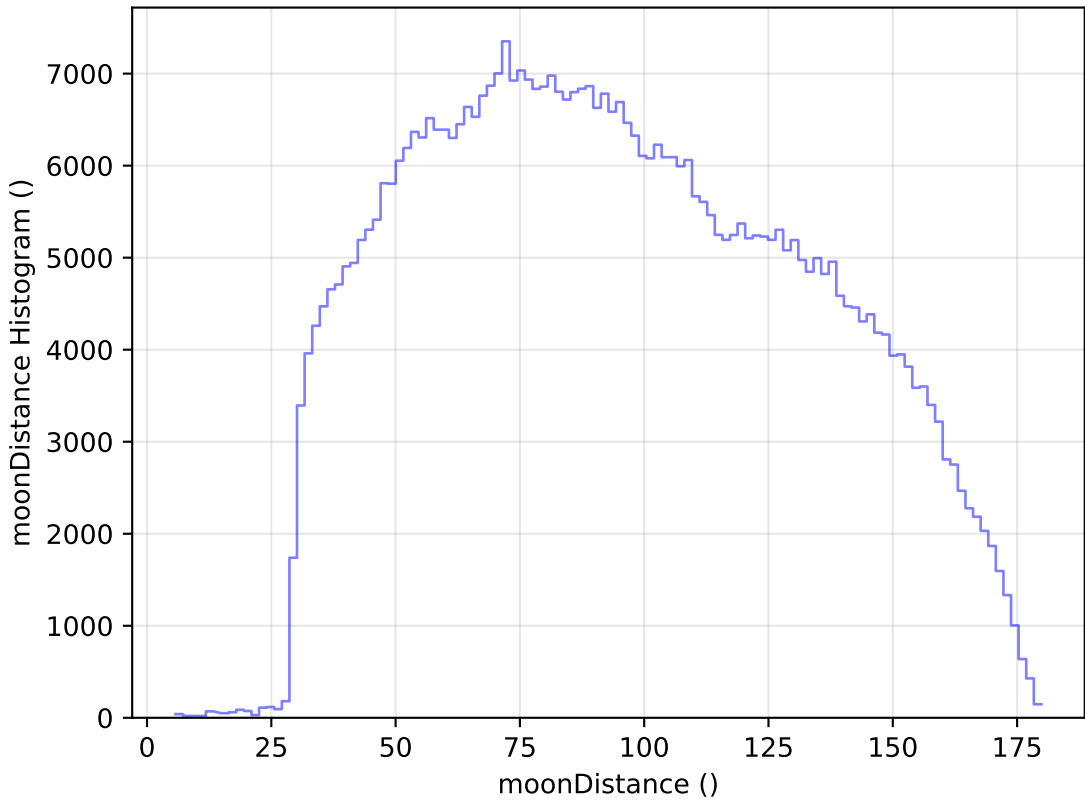
mw_roll_bulge_v3.3_10yrs WFD i band: moonDistance Histogram
