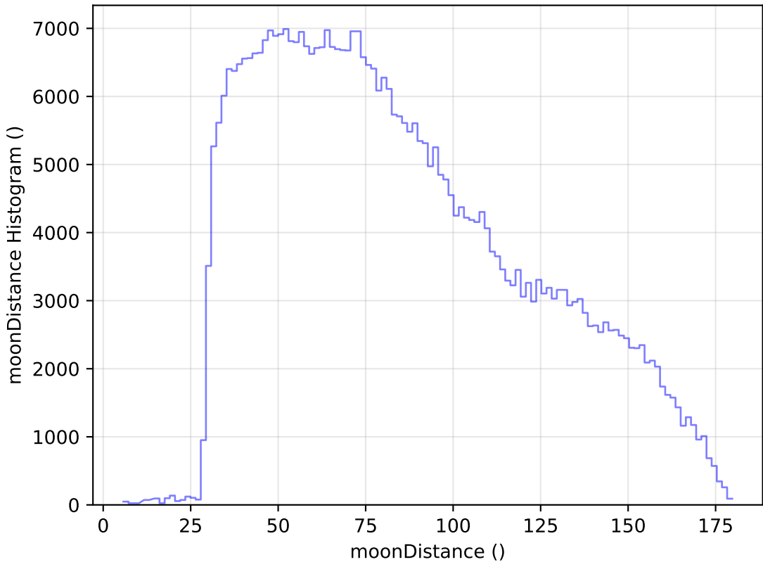
mw_roll_bulge_v3.3_10yrs All sky z band: moonDistance Histogram
