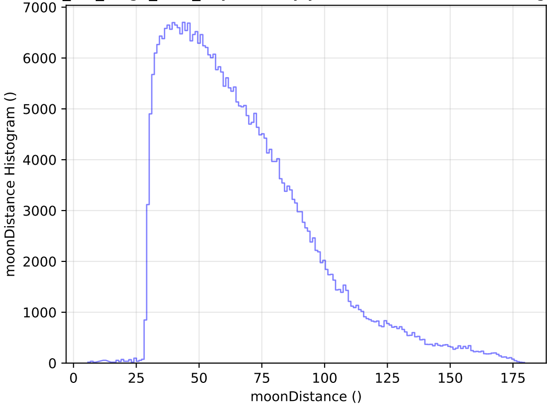
mw_roll_bulge_v3.3_10yrs All sky y band: moonDistance Histogram
