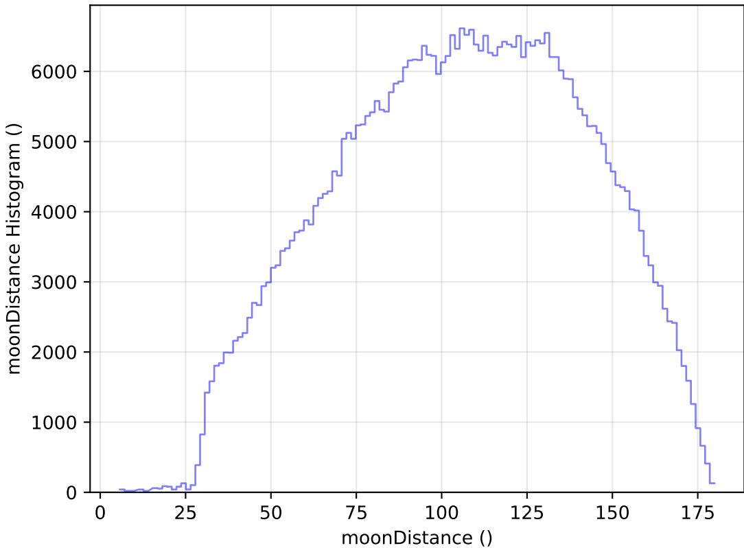
mw_roll_bulge_v3.3_10yrs All sky r band: moonDistance Histogram
