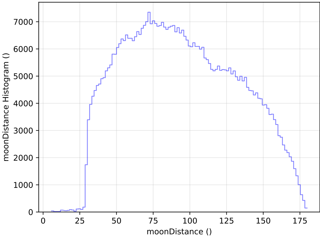
mw_roll_bulge_v3.3_10yrs All sky i band: moonDistance Histogram
