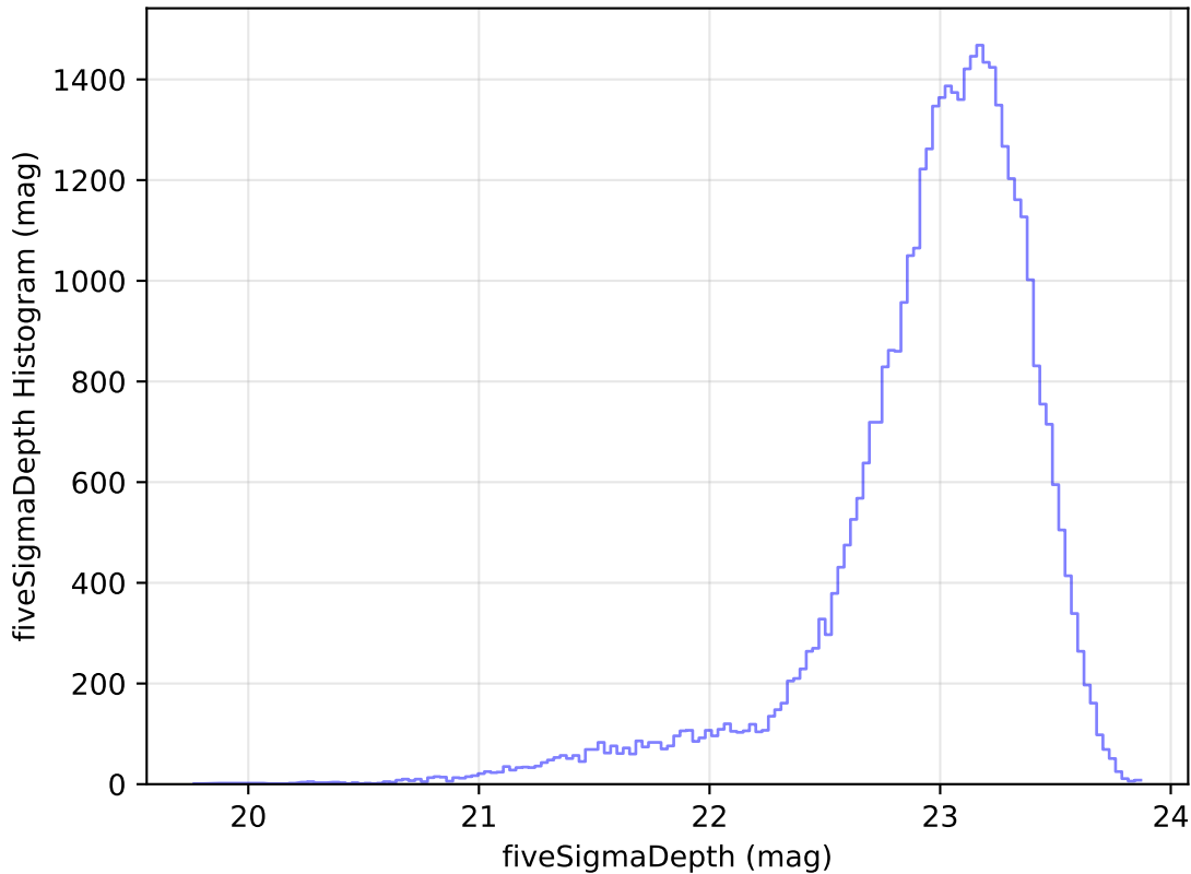
mw_roll_bulge_v3.3_10yrs Yr 1 z band: fiveSigmaDepth Histogram
