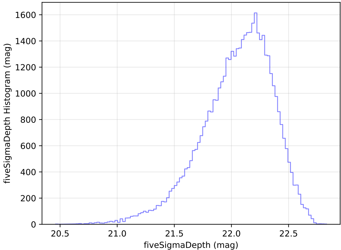
mw_roll_bulge_v3.3_10yrs Yr 1 y band: fiveSigmaDepth Histogram
