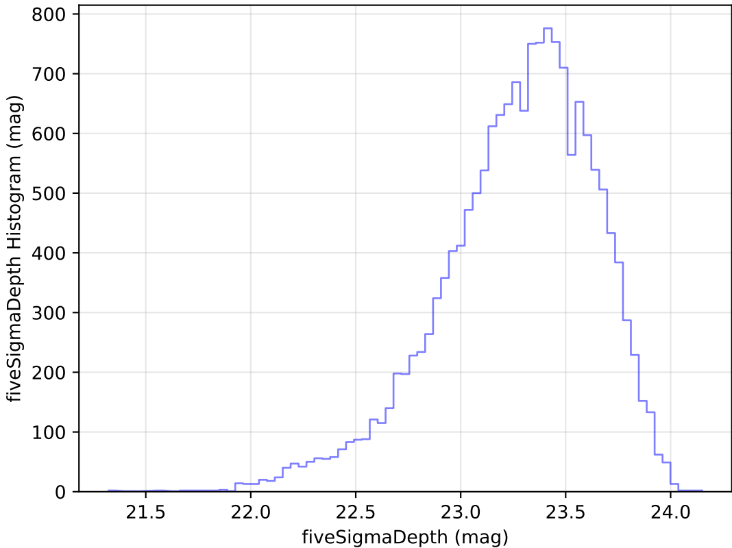
mw_roll_bulge_v3.3_10yrs Yr 1 u band: fiveSigmaDepth Histogram
