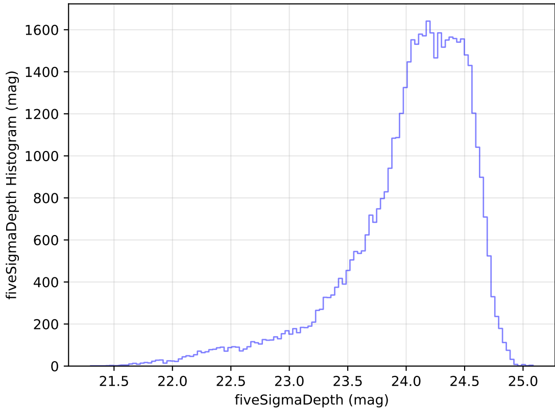
mw_roll_bulge_v3.3_10yrs Yr 1 r band: fiveSigmaDepth Histogram
