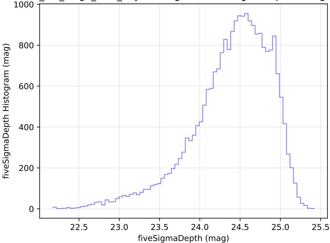
mw_roll_bulge_v3.3_10yrs Yr 1 g band: fiveSigmaDepth Histogram
