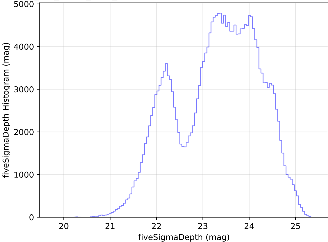
mw_roll_bulge_v3.3_10yrs Yr 1 all bands: fiveSigmaDepth Histogram
