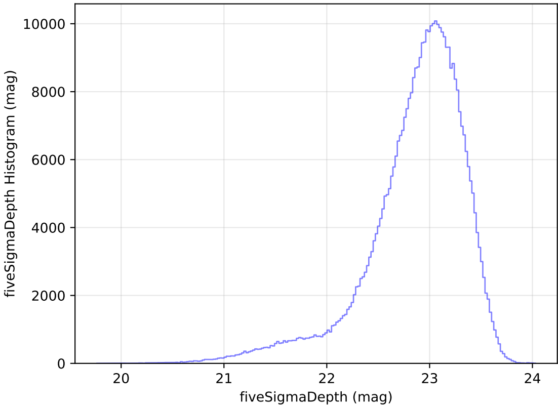
mw_roll_bulge_v3.3_10yrs WFD z band: fiveSigmaDepth Histogram
