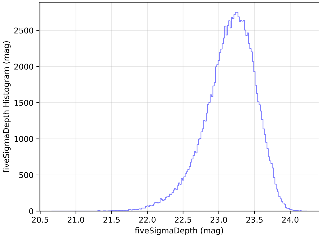
mw_roll_bulge_v3.3_10yrs WFD u band: fiveSigmaDepth Histogram
