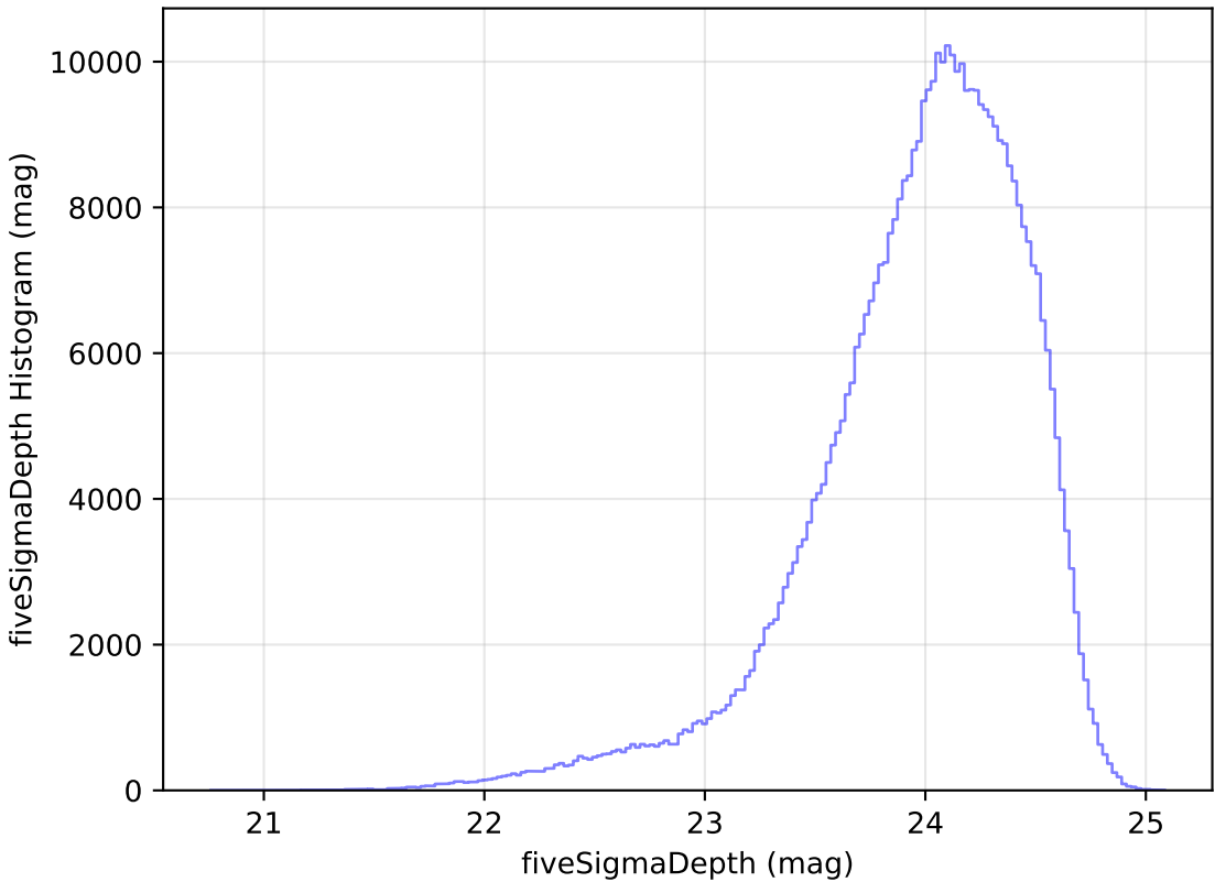
mw_roll_bulge_v3.3_10yrs WFD r band: fiveSigmaDepth Histogram
