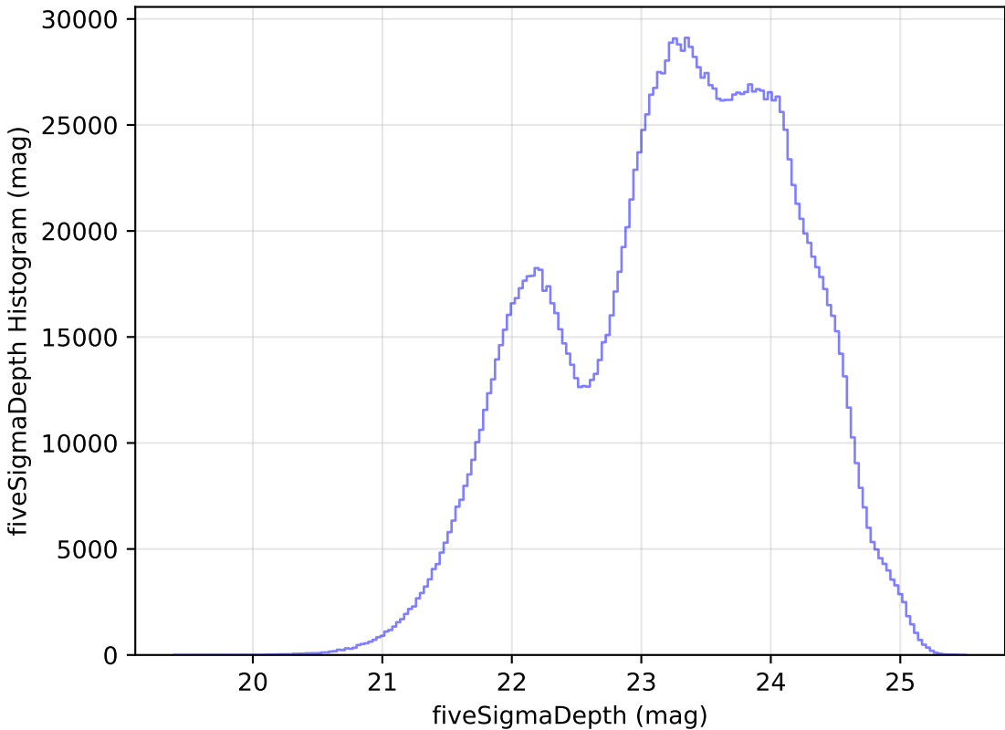
mw_roll_bulge_v3.3_10yrs WFD all bands: fiveSigmaDepth Histogram
