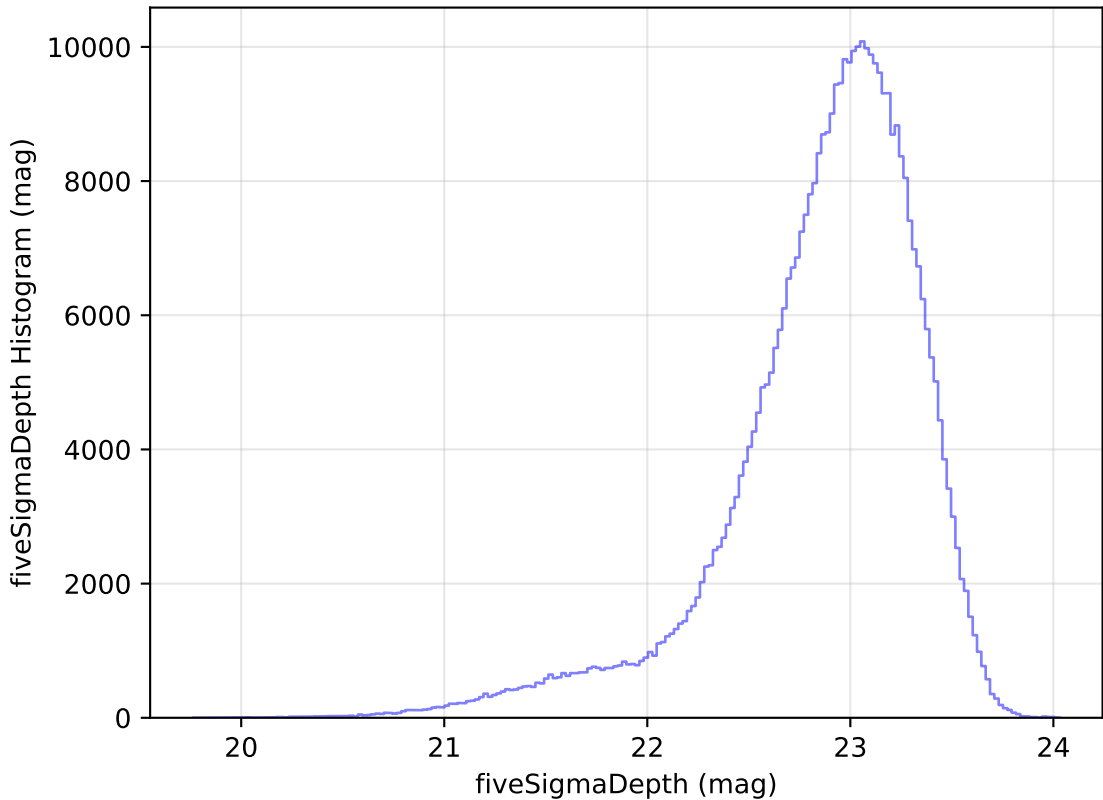
mw_roll_bulge_v3.3_10yrs All sky z band: fiveSigmaDepth Histogram
