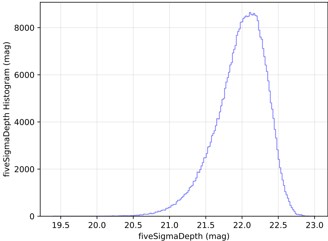
mw_roll_bulge_v3.3_10yrs All sky y band: fiveSigmaDepth Histogram
