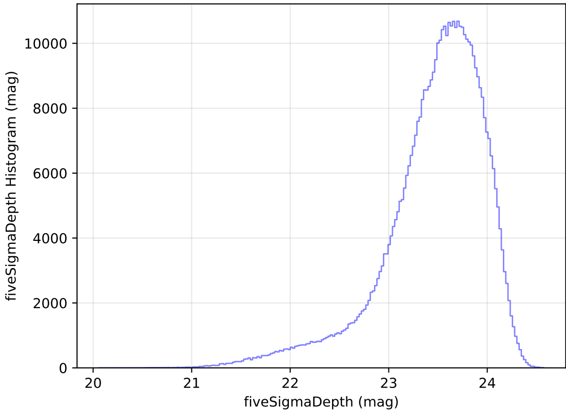
mw_roll_bulge_v3.3_10yrs All sky i band: fiveSigmaDepth Histogram
