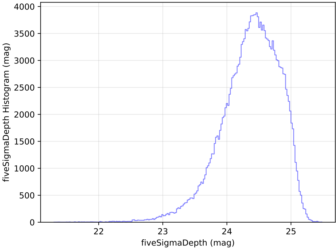
mw_roll_bulge_v3.3_10yrs All sky g band: fiveSigmaDepth Histogram
