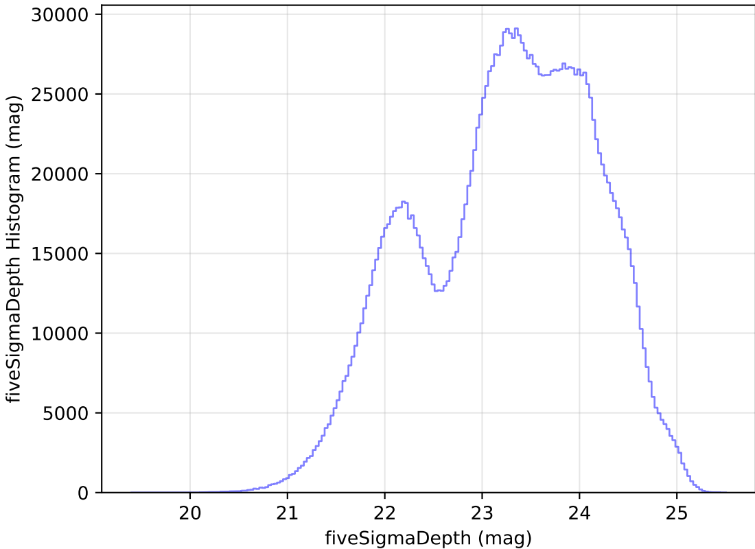
mw_roll_bulge_v3.3_10yrs All sky all bands: fiveSigmaDepth Histogram
