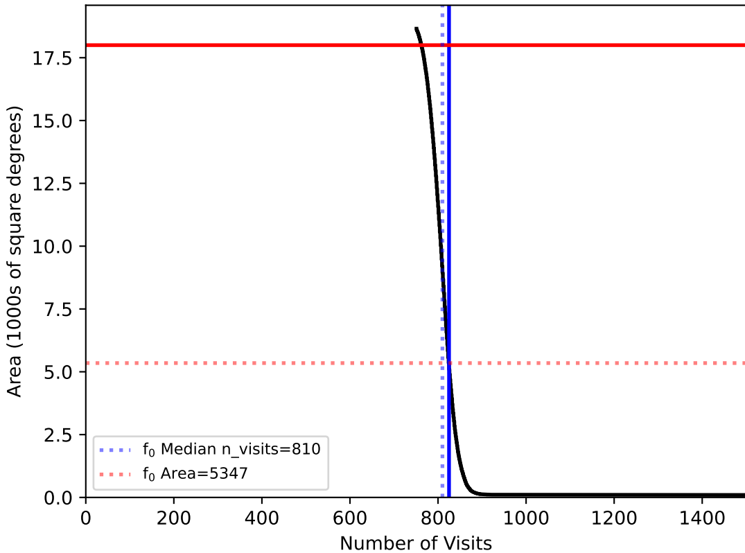
mw_roll_bulge_v3.3_10yrs WFD: f0
